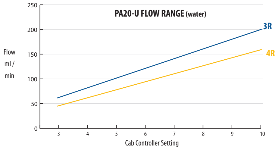
Model PA20-U
